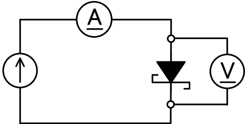
Circuit ①
