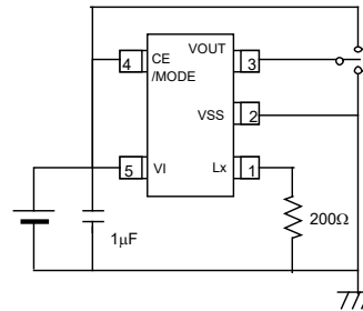
Circuit ②
