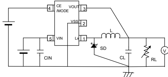
Circuit ①
