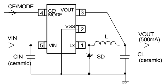
* XC9206/9207/9208 series wire connection
