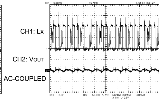
② V_{IN}=4.2V, V_{OUT}=1.8V, I_{OUT}=60mA
