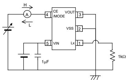
Circuit ⑤
