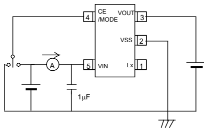
Circuit ③
