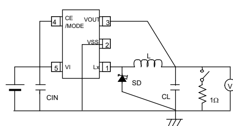
Circuit ⑥
