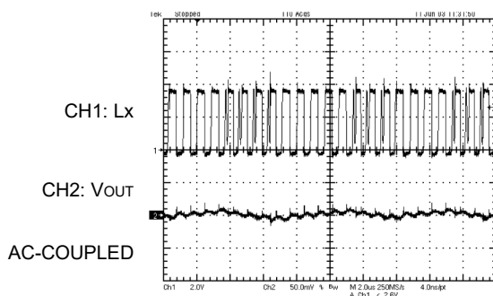
③ V_{IN}=3.6V, V_{OUT}=1.8V, I_{OUT}=30mA
