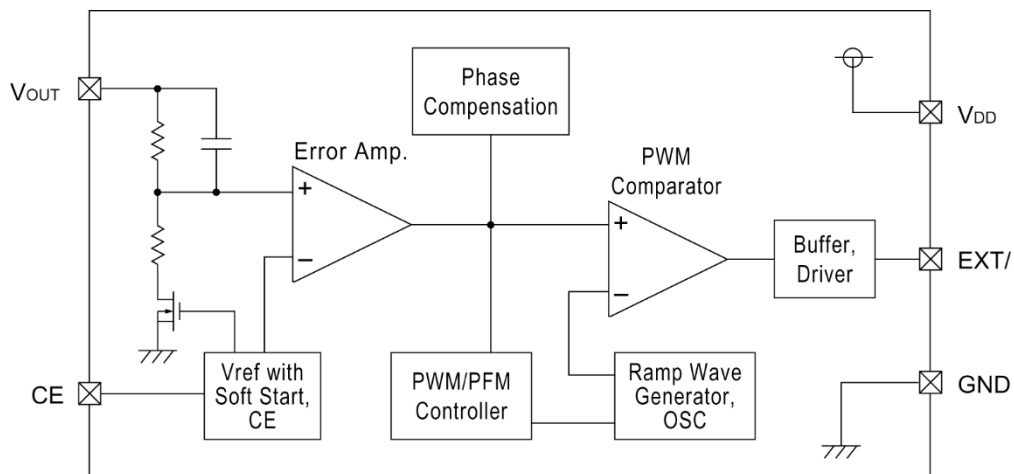
XC6365, XC6366 Series A, C type (VOUT)
