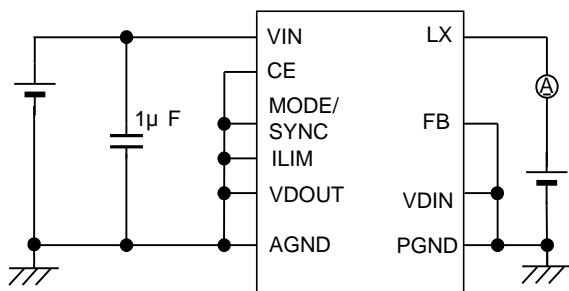
Circuit ⑦
