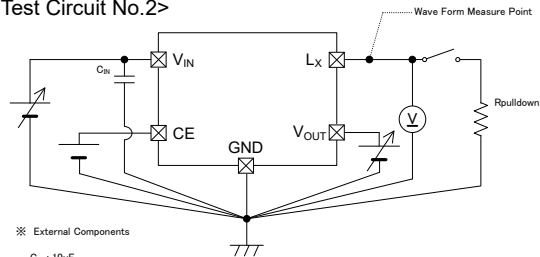
<Test Circuit No.2>
