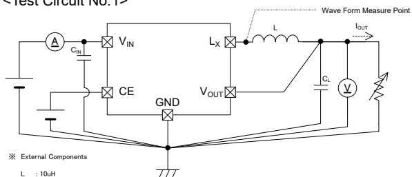
<Test Circuit No.1>
