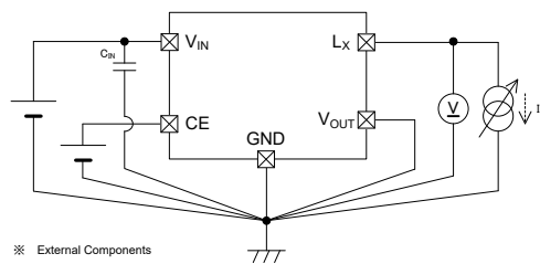
<Test Circuit No.4>
