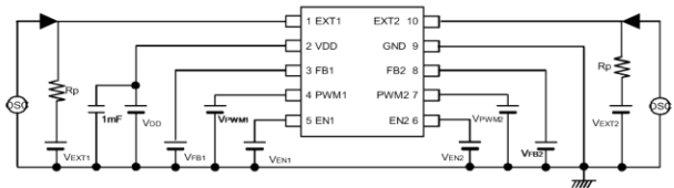
Circuit 6
