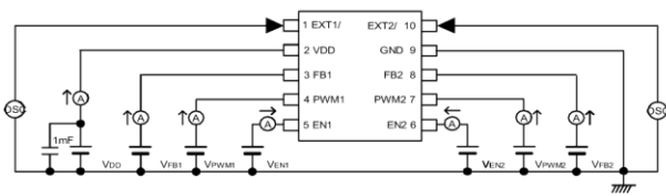
Circuit 3
