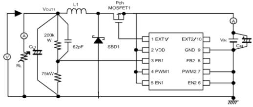
Circuit 4
