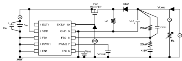
Circuit 6
