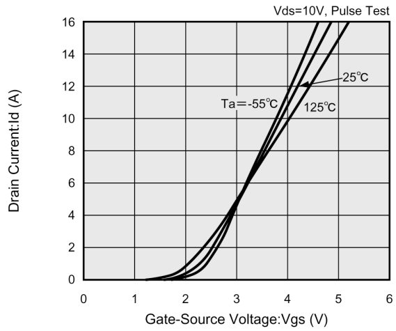
(2) Drain Current vs. Gate-Source Voltage
