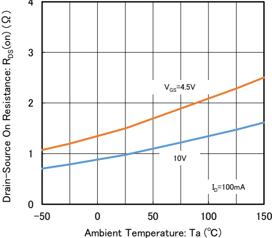
(4) Drain-Source On-State Resistance vs. Ambient Temperature
