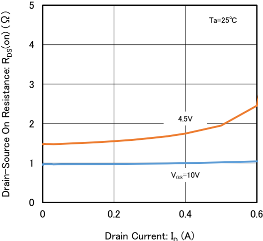
(5) Drain-Source On-State Resistance vs. Drain Current
